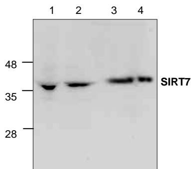
Cat. #: 3099-100SIRT7 Antibody. Western blot analysis of SIRT7 using Jurkat cell lysate (Lane 1 & 2), mouse 3T3 cell lysate (Lane 3) and rat kidney tissue lysate (Lane 4).
