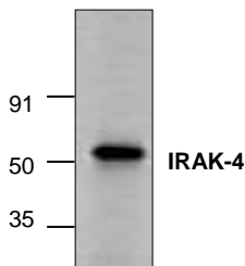
Cat.# 3580-100 Western blot analysis of IRAK-4 expression with HeLa cell lysate.
