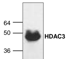
Cat.# 3603-100 Western blot analysis of HDAC3 expression in Jurkat cell lysate.
