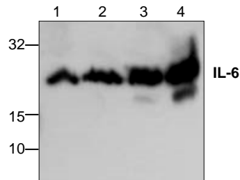
Western blot analysis using recombinant human IL-6.
