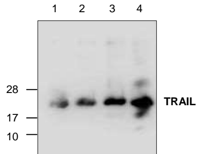
Cat. #: 5354-100 TRAIL Antibody. Western blot analysis using recombinant human TRAIL (Cat.# 4354-10). Lane 1: 50 ng Lane 2: 100 ng Lane 3: 200 ng Lane 4: 500 ng
