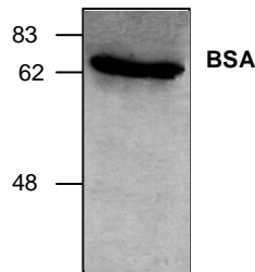
Western Blot analysis with purified BSA.
