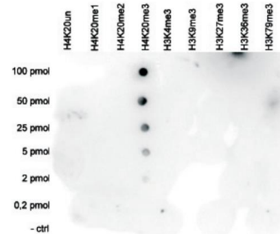
A Dot Blot analysis was performed to test the cross reactivity of the antibody with peptides containing other modifications and unmodified H3 and H4. 100 to 0.2 pmol of the peptide containing the respective histone modification were spotted on a membrane. The Fig shows a high specificity of the antibody for the modification of interest.
