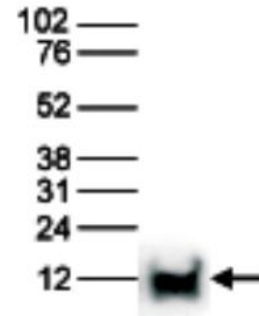
HeLa cells (15 µg) were analysed by Western blot using the antibody. The position of the protein of interest is indicated on the right; the marker (in kDa) is shown on the left.
