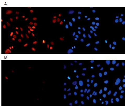
U2OS cells were stained with the antibody and with DAPI. A) The cells were immunofluorescently labelled with the antibody (left) followed by an anti-rabbit antibody conjugated to Alexa568 or DAPI. B) Staining incubation of the antibody with blocking peptide
