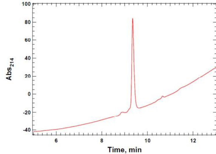
RP-HPLC of Human Recombinant hSUMO2-AMC
